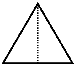
triangle 3 corners 3 sides
