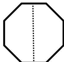
octagon 8 corners 8 sides
